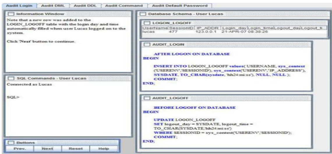
Figure 5. ADbC Database Audit Sub-module: Monitoring User Logins
